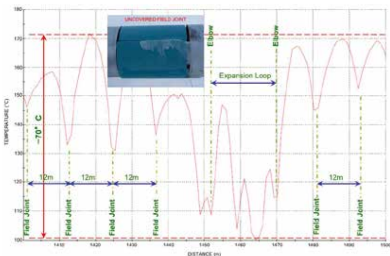
FO Temperature Profile used for Insulation Troubleshooting
